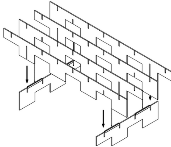
2 - Slot In Long Baffles
